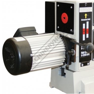
Motor with Belt Change Hand Lever and Lock
